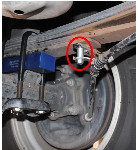
Picture 3: Installation of Hand Brake Cable Bracket Spacer
